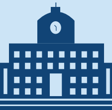
UNC System
